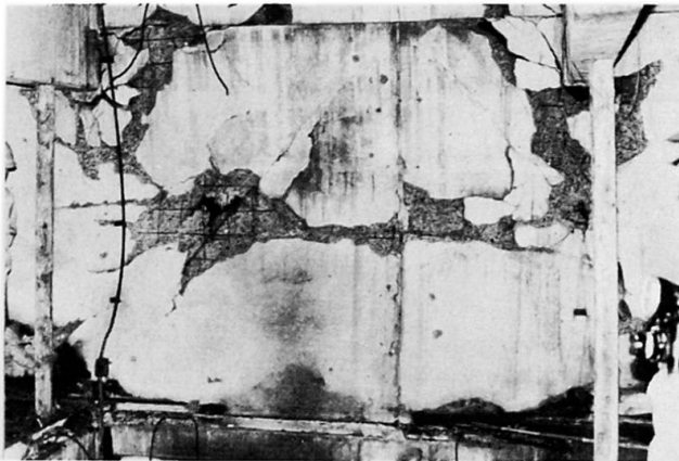
Fig.6 A wall destroyed by gas explosion
