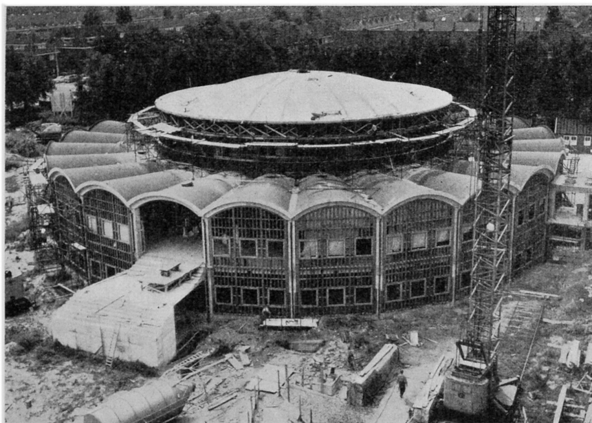
Fig. 7.2 - The rotunda with conical shells and dome.
