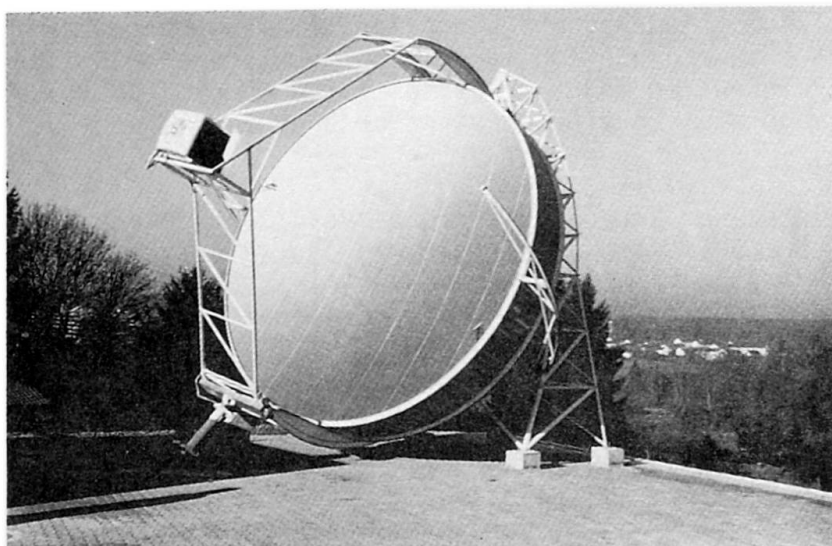
Fig. 10 9 kWe concentrator in Stuttgart
