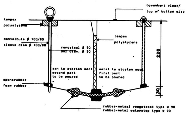
Fig.7 Joint details for joints within and at ends of submersed units.
