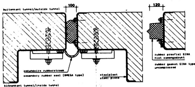
Fig.7 Joint details for joints within and at ends of submersed units.
