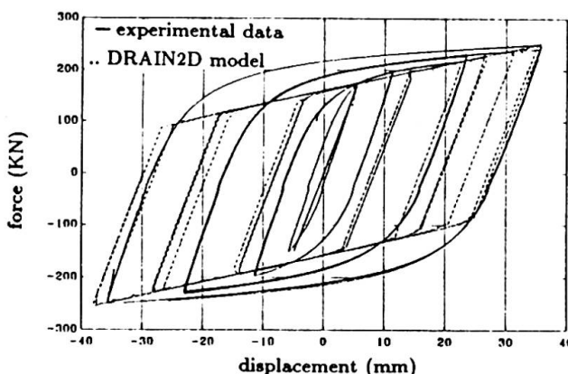
Fig.2 Hysteretic loops of a test beam
