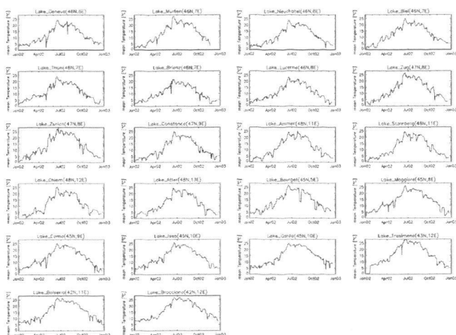
Abbildung 1: Mean average LSWT for the year 2002 of selected lakes in the Alpine region
