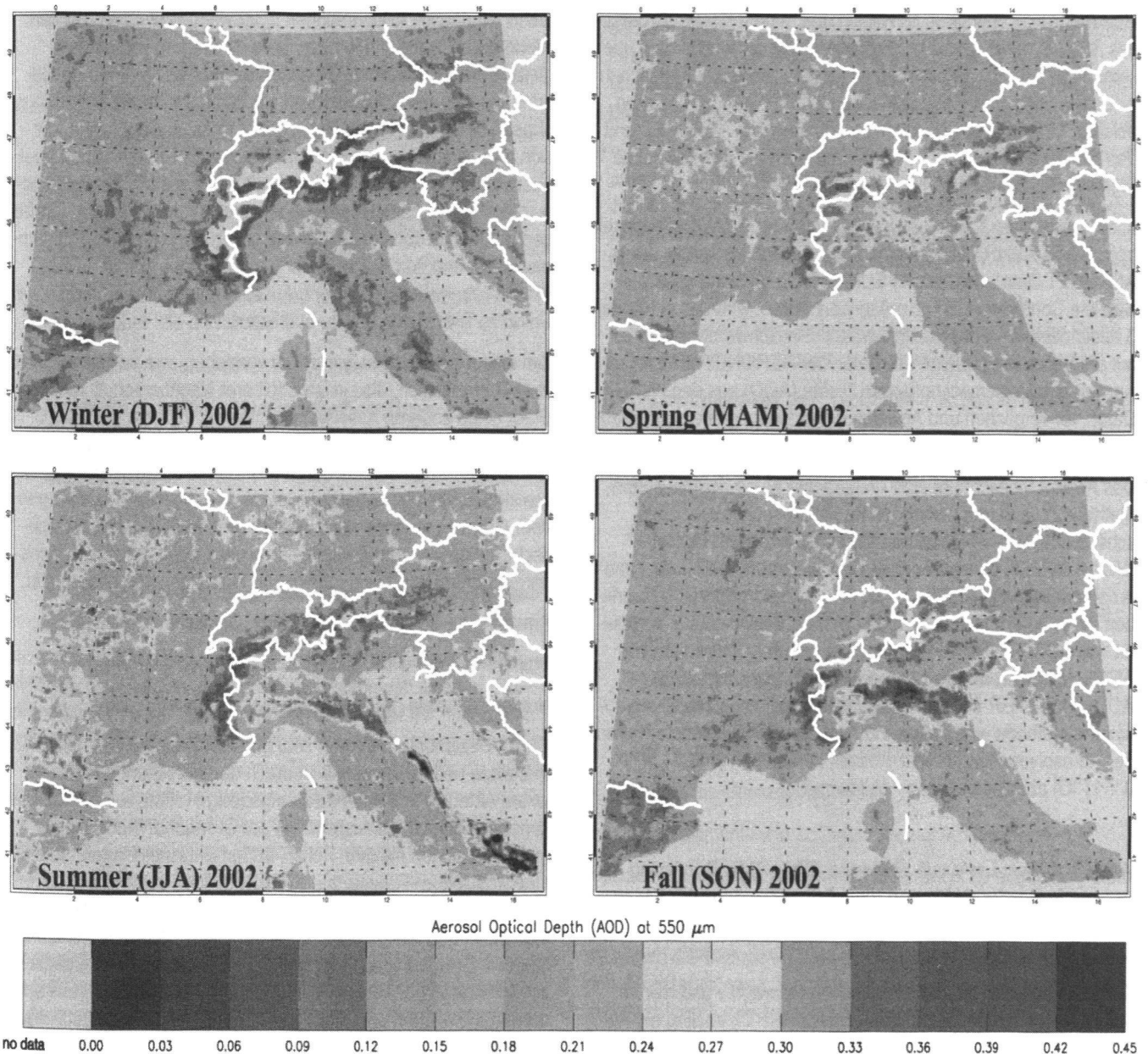
Figure 1: Seasonal (3 months) means of the aerosol optical depth (AOD) in Central Europe in 2002. The images cover the region from 40.5°N to 50°N (1 degree intervals) and from 0°E to 17°E (2 degree intervals). Hauser, A., Oesch, D. and S. Wunderle (2004): NOAA AVHRR derived Aerosol Optical Depth (AOD) over Land: A comparison with AERONET data. – AERONET/PHOTONS workshop, El Arenosillo, Spain, 2004. Journal of the Spanish Society of Optics
