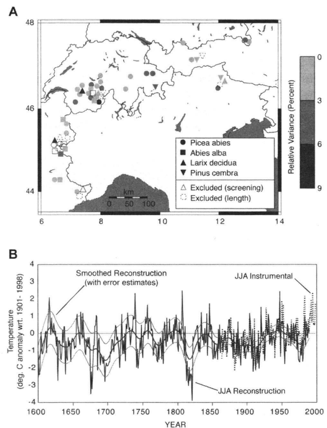
Figure 1. A) Map of the locations of the 53 tree-ring sites used for the reconstruction of June-August and April-September temperatures. Included (shading) is the site weighting in the final model for the 1850-1973 nest for the June-August temperature reconstruction, where it is apparent that the signal is distributed across all species, and the Alpine chain. B) The final June-August temperature reconstruction, derived from splicing the nested models together, is shown for 1600-1989. Also shown are the instrumental temperature data and the smoothed reconstruction. Error estimates for the smoothed reconstruction were defined by \pm the root-mean-squared-error between the model nests and independent verification data. Prior to the summer of 2003 (not shown), the summer of 1807 is reconstructed to be the warmest summer since 1600. Coolest conditions occur about a decade later, which are likely related to the Dalton minima in solar activity and cooling following significant volcanic eruptions, including Tambora (1815), around this time.
