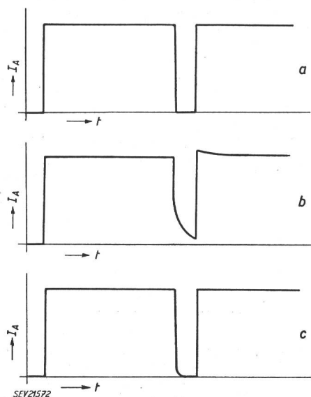
Fig. 12 Signalformen
