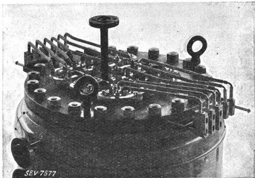
Fig. 4. Oelheizkessel (Anschlüsse).
