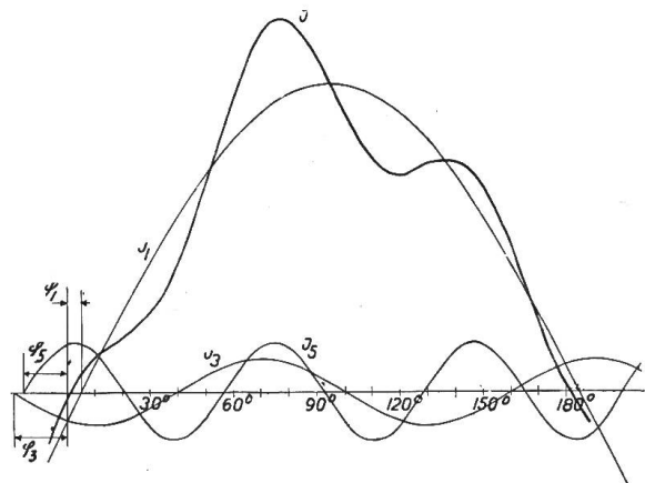
Fig. 7d \varphi_1 = 5^\circ, \varphi_3 = 20^\circ, \varphi_5 = 16,5^\circ
