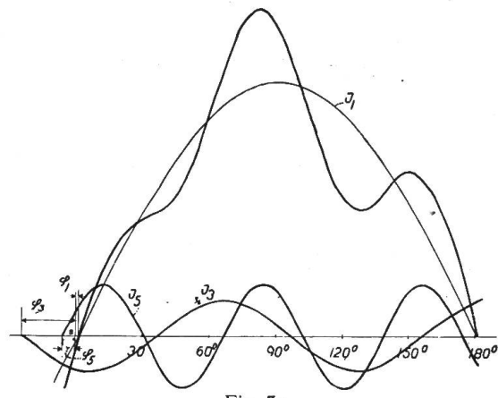
Fig. 7c \varphi_1 = 1^\circ, \varphi_3 = 24^\circ, \varphi_5 = 6,4^\circ
