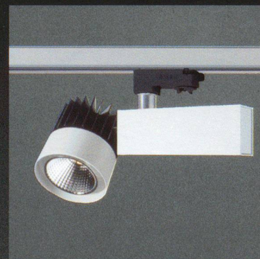
MITRON 41.2W / 2350lm LED spot per binario
