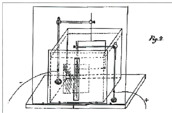
Fig. 4. Electrochemical actinometer wooden box (original engraving).
