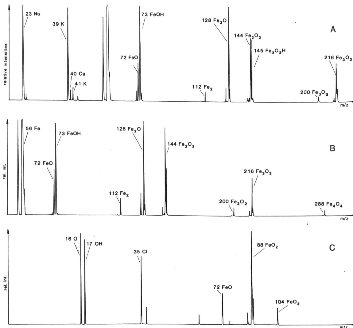
FIG. 6. — LAMMA spectra recorded for particles obtained from the "meteorite" collected in Brittany. A and B recorded in the positive mode, C in the negative mode.
