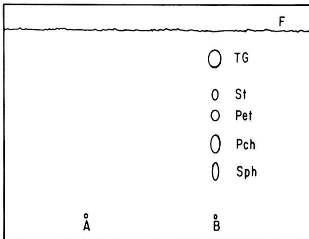
Fig. 3. Detection of lipid peroxides by thin-layer chromatography. T. cruzi epimastigotes were preincubated in the presence of 100 \mu\text{M} rose bengal for 60 min in the dark, and for 10 min under illumination as described in "Materials and Methods" section. Samples of cell suspensions were extracted and treated as described (Stahl, 1958). The chromatograms were developed by the starch-iodide procedure of Stahl (1958) to visualize the peroxides. (A) Control cells incubated in the absence of rose bengal. (B) Rose bengal-treated cells. Abbreviations used: Sph = sphingomyelin; Pch = phosphatidylcholine; Pet = phosphatidylethanolamine; St = sterols; TG = triacylglycerols.
