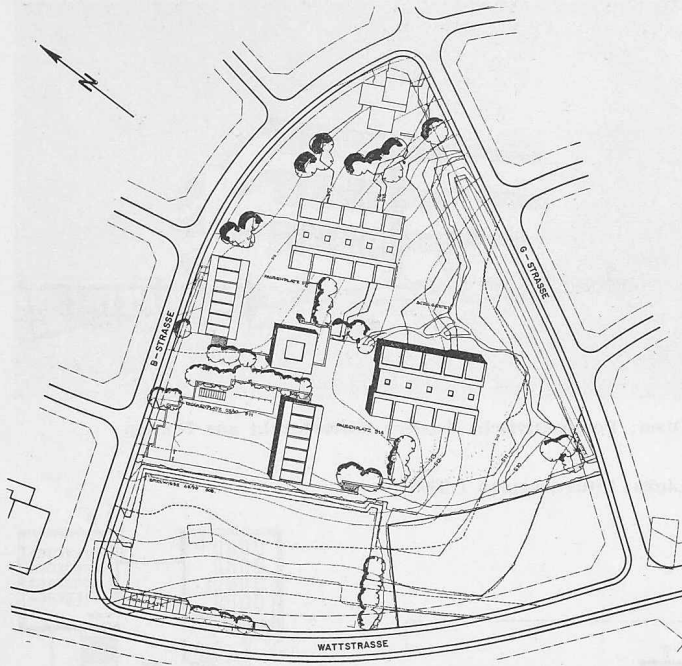
Situationsplan 1:3000
