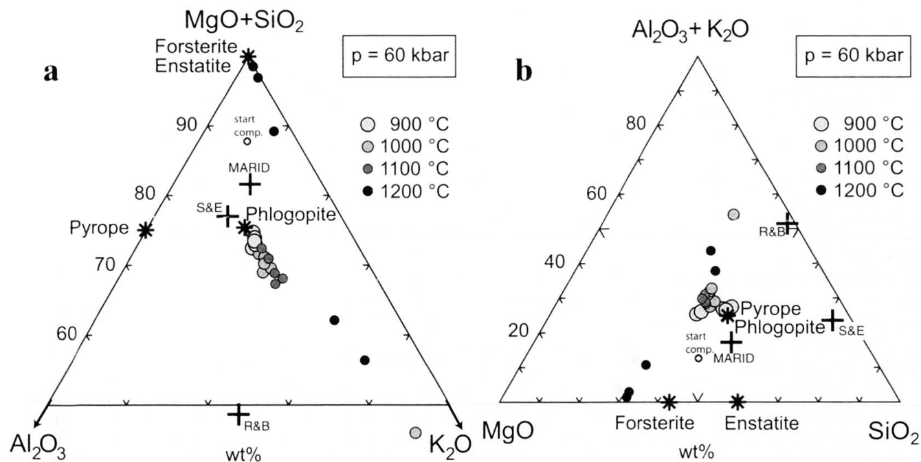
Fig. 2 Composition of the dry solute in the run series forsterite-phlogopite-H 2 O at 60 kbar: (a) \text{MgO}+\text{SiO}_2 - \text{Al}_2\text{O}_3 - \text{K}_2\text{O} ternary diagram (wt%) and (b) \text{Al}_2\text{O}_3+\text{K}_2\text{O} - \text{MgO} - \text{SiO}_2 ternary diagram (wt%). For explanations see Fig. 1.
