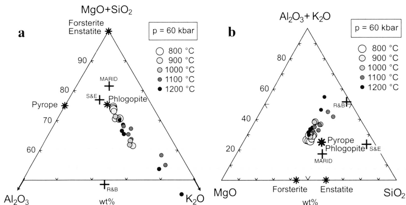
Fig. 1 Composition of the dry solute in the run series phlogopite-H 2 O at 60 kbar projected from H 2 O: (a) \text{MgO}+\text{SiO}_2 - \text{Al}_2\text{O}_3 - \text{K}_2\text{O} ternary diagram (wt%) and (b) \text{Al}_2\text{O}_3+\text{K}_2\text{O} - \text{MgO} - \text{SiO}_2 ternary diagram (wt%). Results from previous studies at 11 kbar and 1100 °C (R&B; RYABCHIKOV and BOETTCHER, 1980) and 20 kbar and 1100 °C (S&E; SCHNEIDER and EGGLE, 1986) are plotted for comparison. Between 10 and 20 kbar the silica contents in the fluid increases markedly (b), followed by an increase in MgO to 60 kbar. As the absolute solute content in the fluid (not shown in this figure) strongly increases between 20 and 60 kbar, the absolute silica contents in the fluid do not decrease. The approximate composition of a MARID-nodule (SWEENEY et al., 1993) is also shown (FeO was calculated as MgO). Except for the data at 20 kbar (S&E), which are too silica-rich, MARID could be produced by a reaction of forsterite+enstatite with a potassic fluid.
