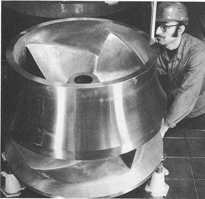
Pumpenrotor (halbradial)
