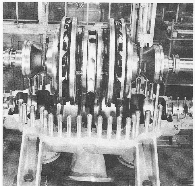
Pumpenrotor (radial)
