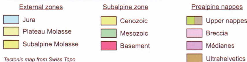
Tectonic map from Swiss Topo
