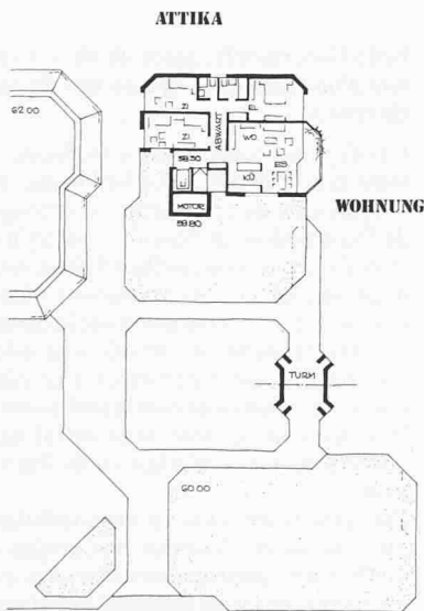
Grundriss Attikageschoss 1 : 700
