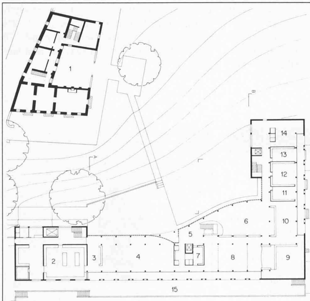
Piano terra 1:700
