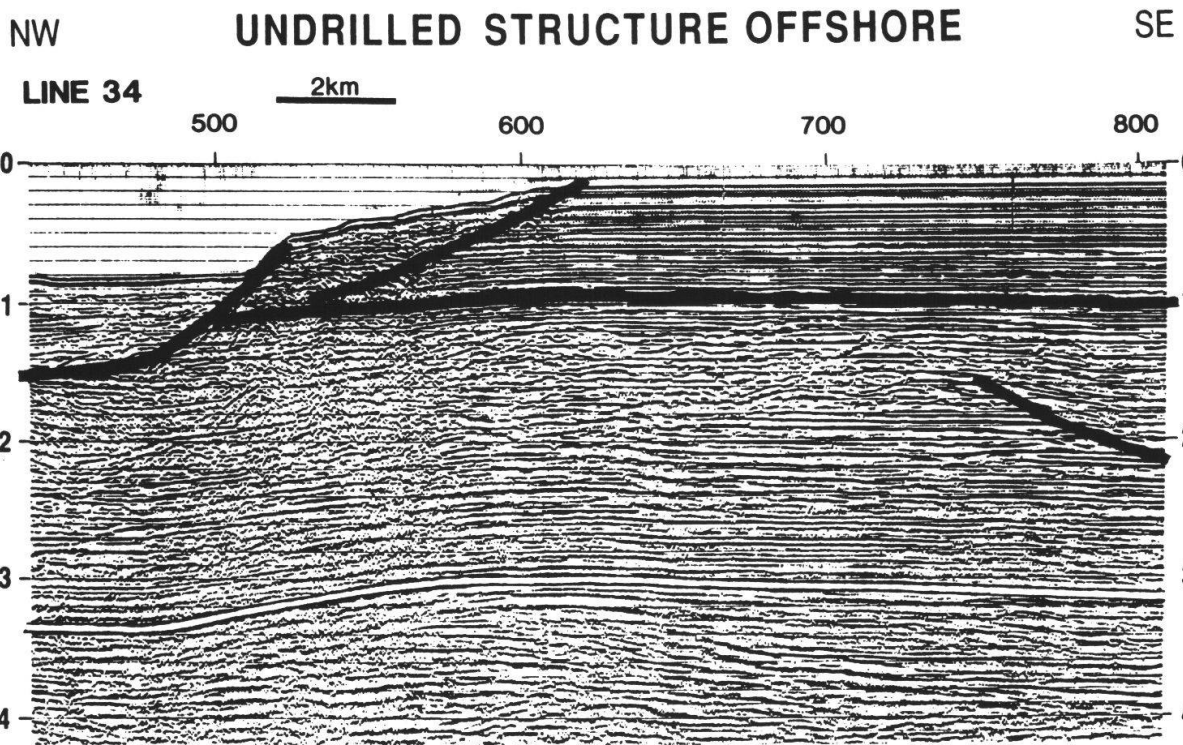
Fig. 3a: Seismic line 34 with undrilled offshore structure under E shoulder of Swatch of No Ground, with Petrobangla interpretation (from PETROBANGLA 1993).
