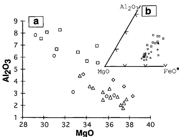
Fig. 4 Chemical diagrams for serpentinized peridotites from Pelvas d'Abriès (PL) and Montgenèvre (MOC). (a) \text{Al}_2\text{O}_3\text{-MgO} diagram clearly showing a negative linear correlation and two distinct fields for the ultrabasic rocks from PL and for those from MG. This difference may be partly explained by the presence of chromiferous spinel and interstitial chloritized plagioclase within the Pelvas samples. (b) \text{MgO-Al}_2\text{O}_3\text{-FeO}^* diagram underlying the chemical difference between PL and MOC peridotites. (c) \text{V-Cr} diagram showing good linear trends of the representative points from both localities. The higher Cr contents of the PL ultrabasic intrusive rocks are linked to the presence of the chromiferous spinel.
