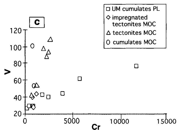
Fig. 4 Chemical diagrams for serpentinized peridotites from Pelvas d'Abriès (PL) and Montgenèvre (MOC). (a) \text{Al}_2\text{O}_3\text{-MgO} diagram clearly showing a negative linear correlation and two distinct fields for the ultrabasic rocks from PL and for those from MG. This difference may be partly explained by the presence of chromiferous spinel and interstitial chloritized plagioclase within the Pelvas samples. (b) \text{MgO-Al}_2\text{O}_3\text{-FeO}^* diagram underlying the chemical difference between PL and MOC peridotites. (c) \text{V-Cr} diagram showing good linear trends of the representative points from both localities. The higher Cr contents of the PL ultrabasic intrusive rocks are linked to the presence of the chromiferous spinel.
