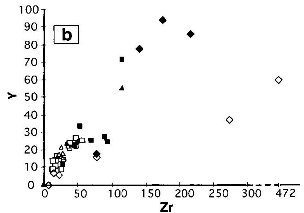
Fig. 3 Chemical diagrams for gabbro types from Pelvas d'Abriès (PL), Montgenèvre (MOC) and Rocciavre (ROC). (a) \text{TiO}_2\text{-MgO} diagram. Note the large contrast in the distribution mode of the Ca-Mg and Fe-Ti gabbro representative points. (b) \text{Y-Zr} diagram. Low concentrations for most analyzed samples contrast with significantly higher concentrations of several samples from MOC.
