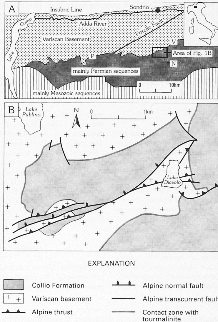
Fig. 1. (A) Simplified geologic map of the Orobic Alps showing location of the study area (box); N = Novazza uranium mine, P = Lake Pescegallio, V = Val Vedello uranium mine. (B) Sketch map of the geology near Lake Publino and Lake Diavolo showing tourmalinite settings. Modified from ZHANG et al. (1994).
