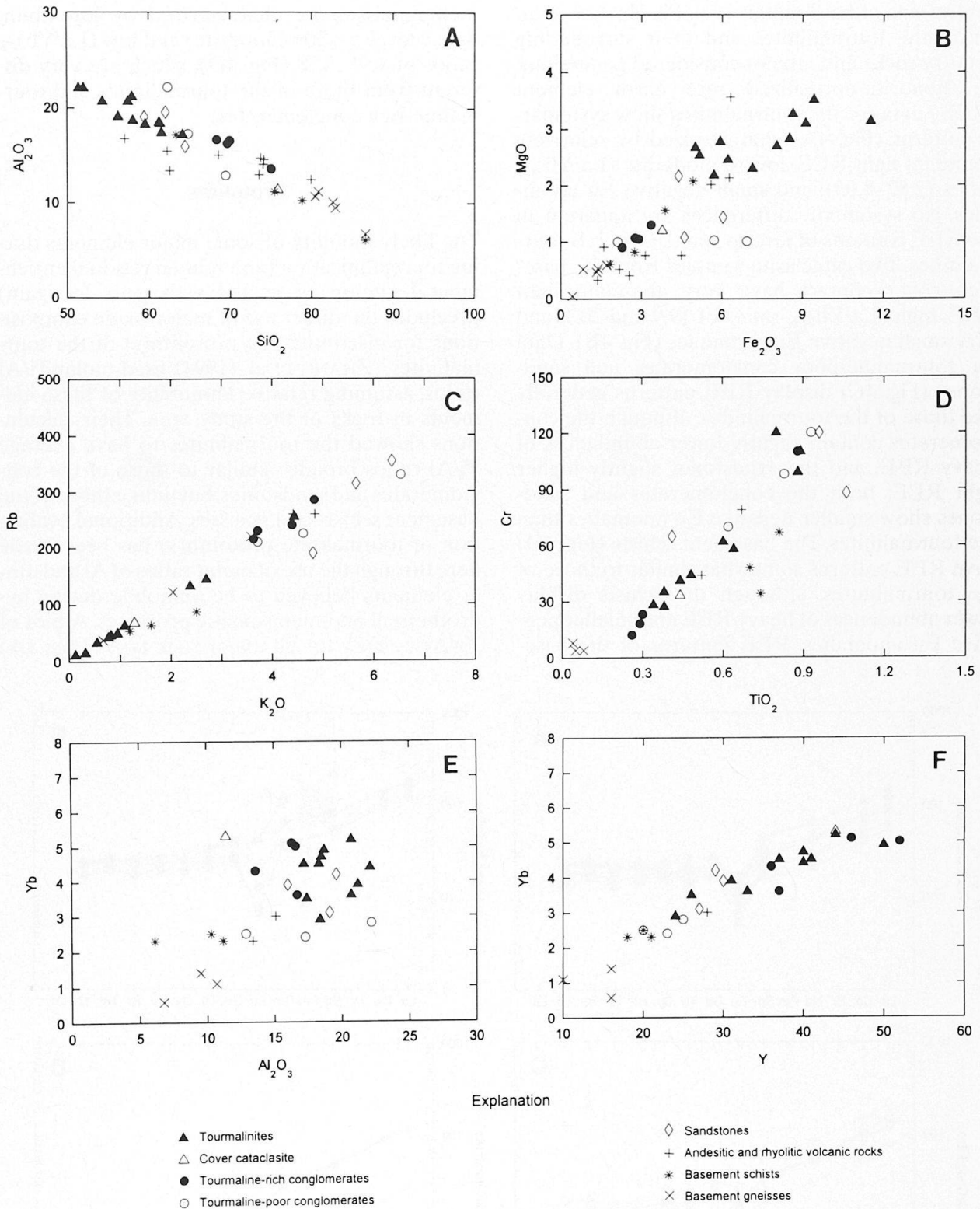
Fig. 3 Variation diagrams showing correlations of whole-rock analytical data. (A) SiO 2 vs Al 2 O 3 ; (B) Fe 2 O 3 vs MgO; (C) K 2 O vs Rb; (D) TiO 2 vs Cr; (E) Al 2 O 3 vs Yb; (F) Y vs Yb. Major element values in wt%, trace elements in ppm; Fe 2 O 3 in (B) is total iron. Data for volcanic rocks from this study and CADEL (1986).
