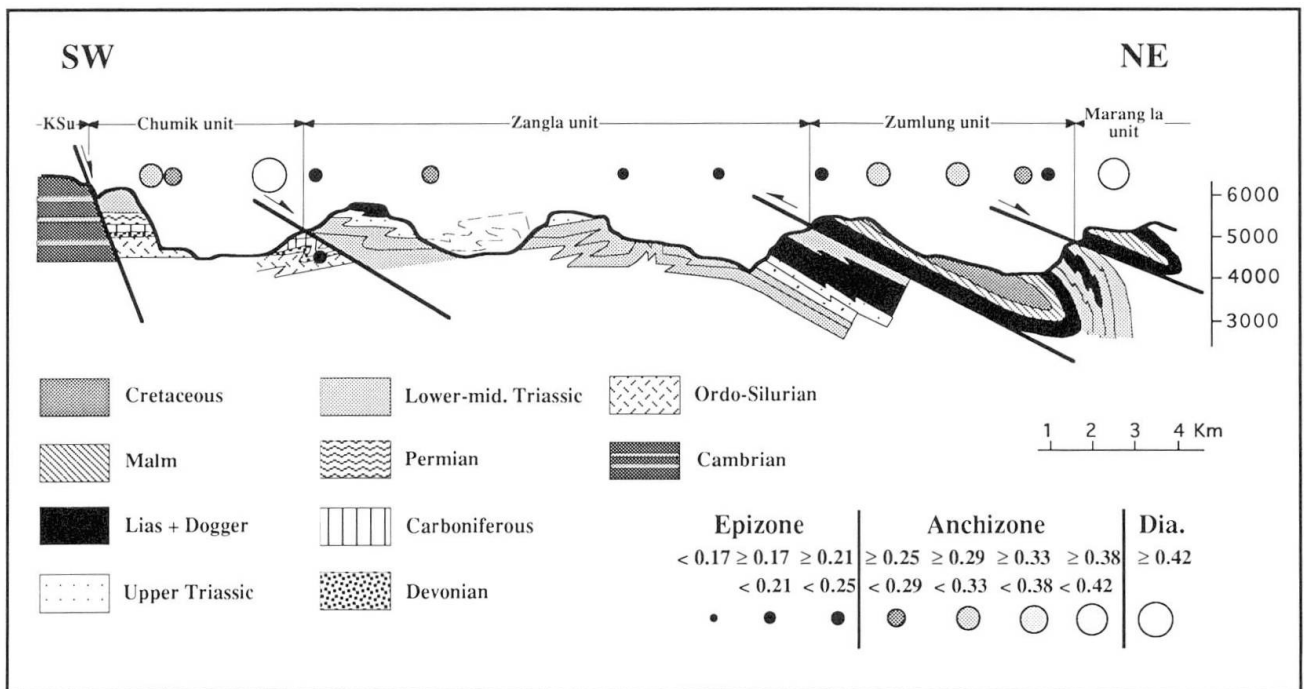
Fig. 5 Cross-section through the tectonic units of the Tibetan zone in SE Zaskar. Location in figure 1. The IC values for the Zumlung and Marang la units are own unpublished data.
