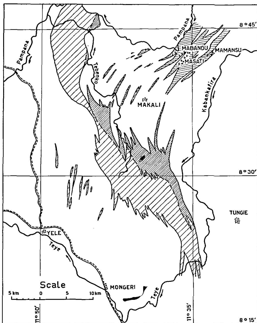
Fig. 1. The schistbelt of the Kangari Hills and the Masati area in Central Sierra Leone.
