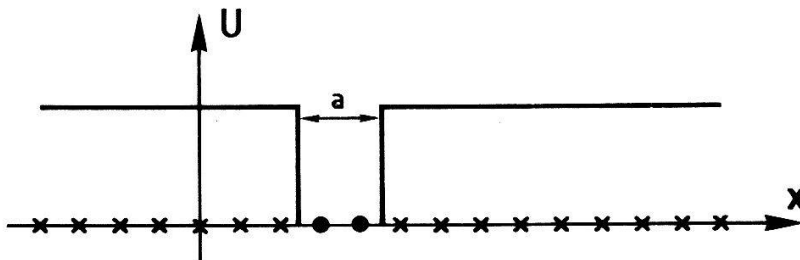
Fig. 5 Potential well
