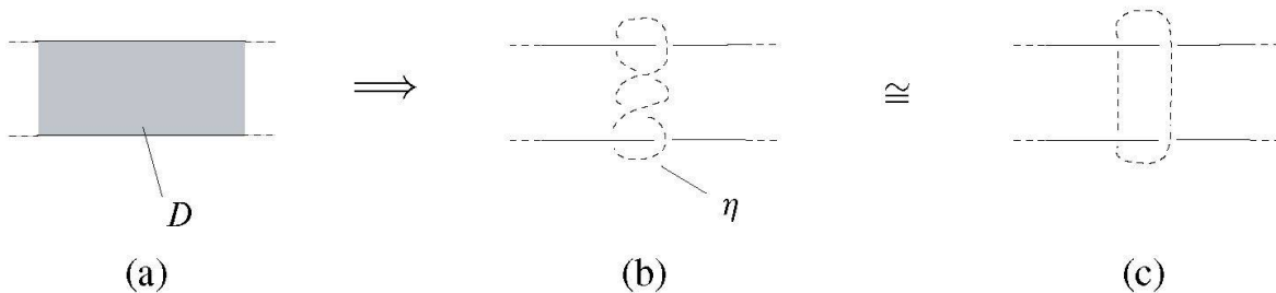
Figure 4.1. Infection by a knot.
