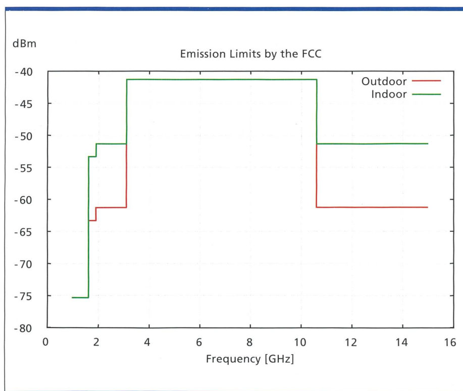
Fig. 1. Graphical representation of the emission limits for UWB communication applications. Note that the outdoor limits are lower than the indoor limits in order to protect incumbent radio services [2].
