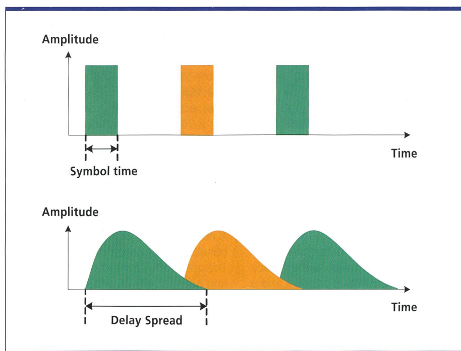
Fig. 2. When a signal is sent at a high rate over a time-dispersive channel (which is typically the case for Broadband Wireless Access), successive symbols suffer from Inter-Symbol-Interference (ISI).
